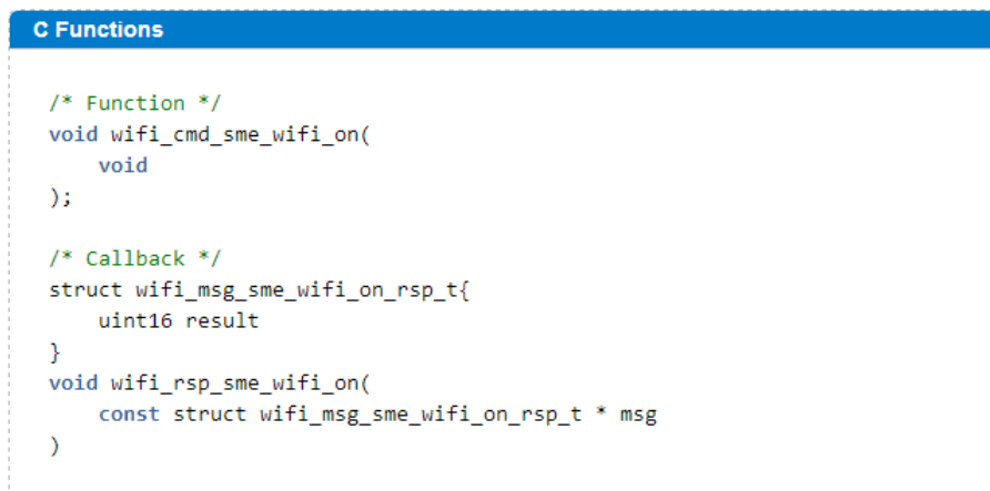
Figure 6: BGLib C functions and call backs
