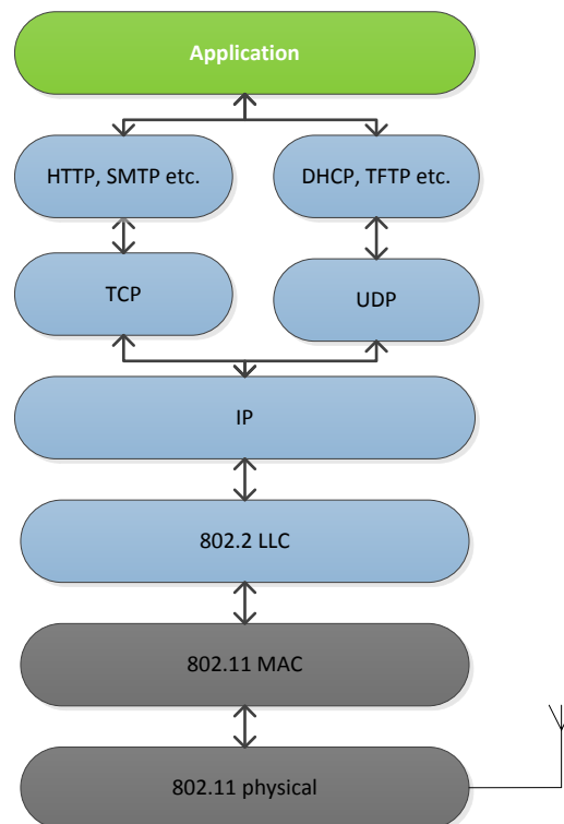
Figure 1: 802.11 and Internet protocol architecture
